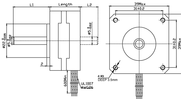
外形图(Dimension):
