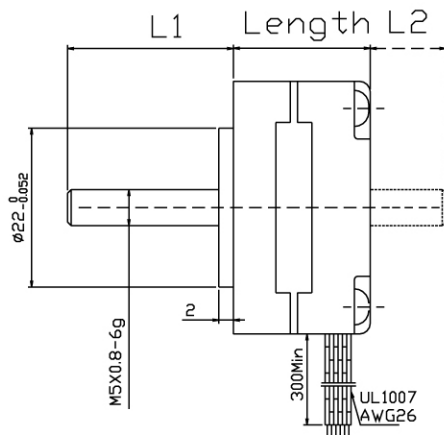
外形图(Dimension):
