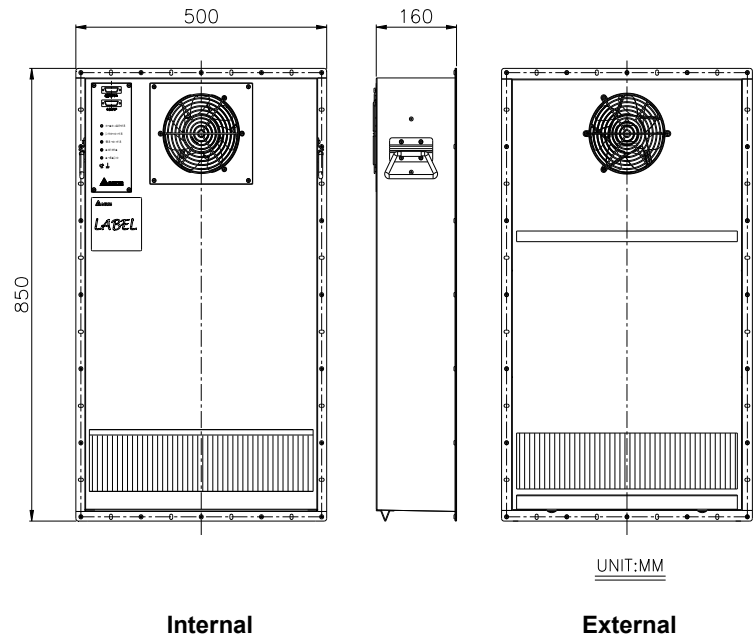
Dimension drawing
